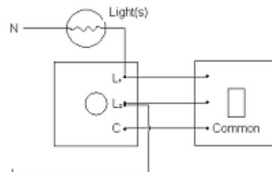
Figure 4 Using a 2-way Dimmerswitch
